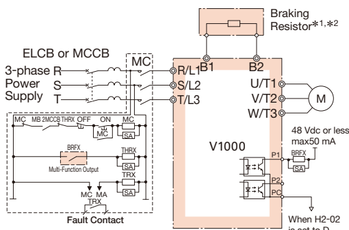
Connection Diagram A
