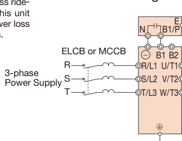
Connection Diagram
