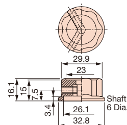
Dimensions (mm)
