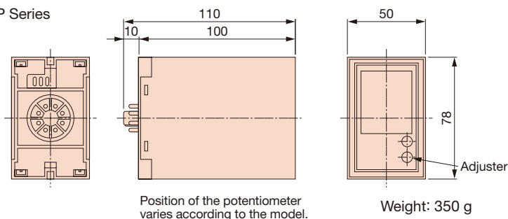
Dimensions (mm)
