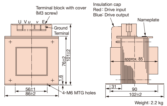
Dimensions (mm)
