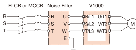
Noise Filter [Schaffner Elektronik AG]
