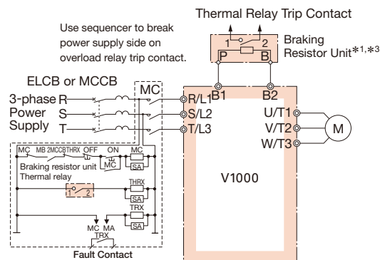
Connection Diagram B
