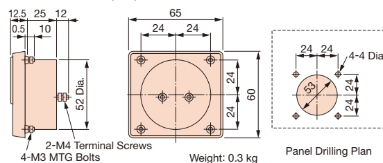
Dimensions (mm)
