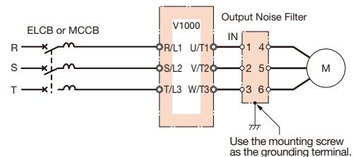
Connection Diagram
