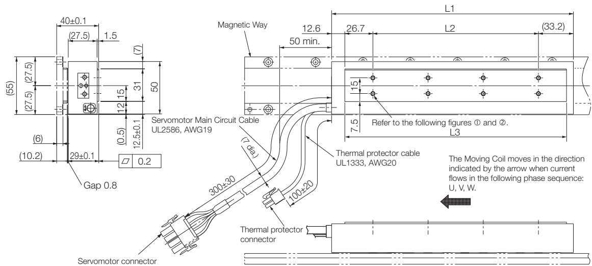
① SGLFW2-30A120AT
