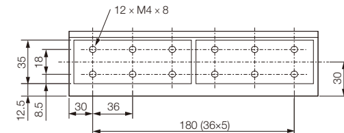
②SGLFW-35A230A□□D
