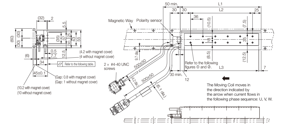
①SGLFW-35A120A□□D
