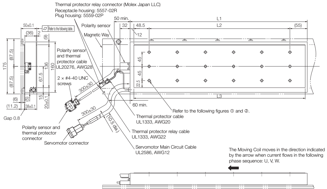
②SGLFW2-1DA560AS
